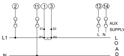
d) 1 Phase 2 Wire Unbalanced Load
