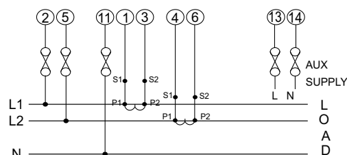
c) 1 Phase 3 Wire Unbalanced Load
